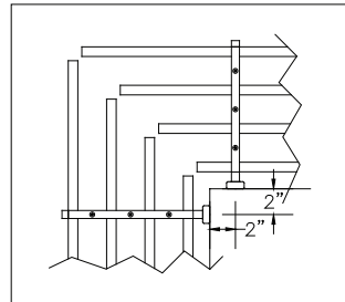
Exterior Mitred Corner
