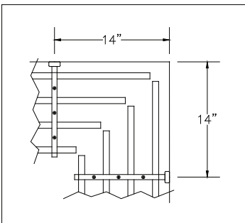
Interior Mitred Corner
