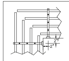
Exterior Mitred Corner
